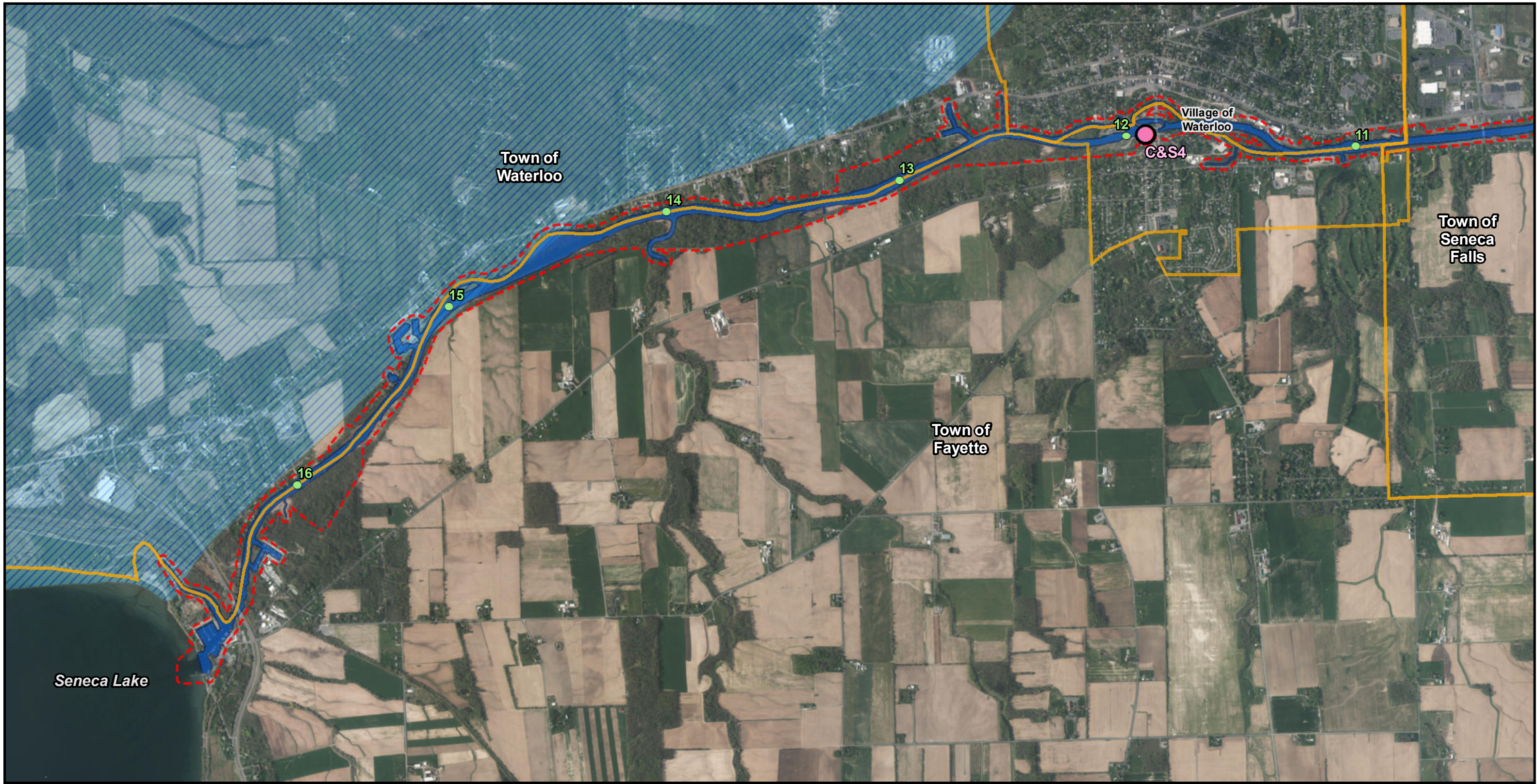
Figure 90F: Aquifers
